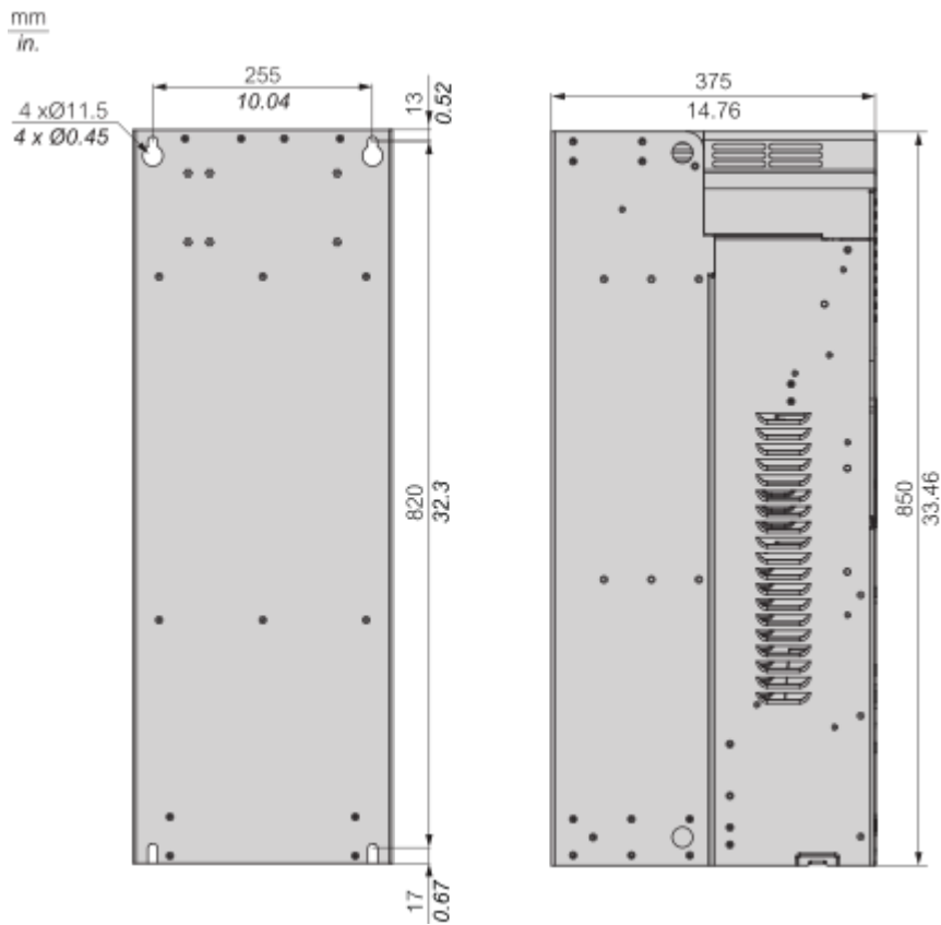
IP20 Drives - Front and Rear View With Conduit Box
