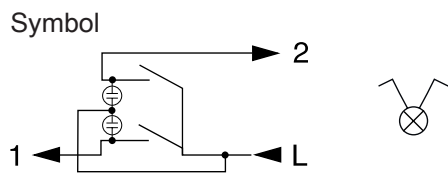
Two-circuit switch with locator light
